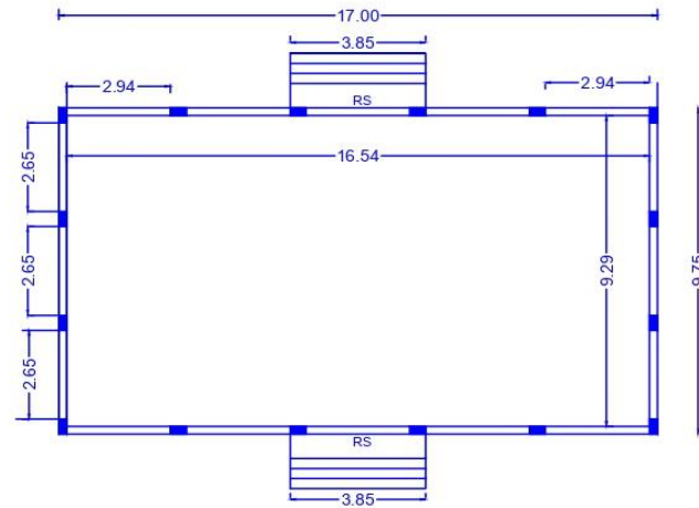
PLAN SCALE 1:100
